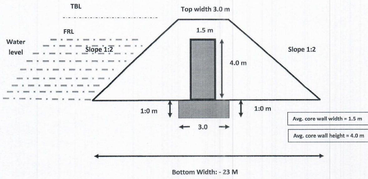
Schematic Diagram of Earthen Dam
